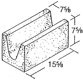
Figure 13-1 8 x 8 x 16 Beam Lintel
