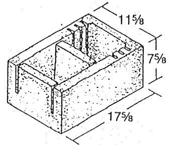
Figure 13-6 12 x 8 x 18 Bond Beam With Knockouts *
