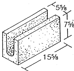
Figure 13-8 6 x 8 x 16 Beam Lintel *
