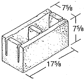
Figure 13-4 8 x 8 x 18 Bond Beam With Knockouts *
