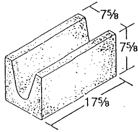
Figure 13-2 8 x 8 x 18 Beam Lintel *
