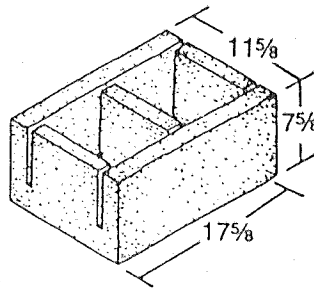
Figure 13-5 12 x 8 x 18 Bond Beam With Knockouts *
