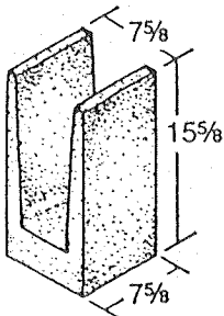
Figure 13-7 8 x 8 x 16 Soldier Course Beam Lintel *
