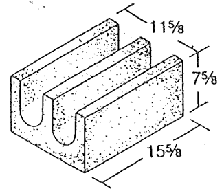
Figure 13-3 12 x 8 x 16 Beam Lintel
