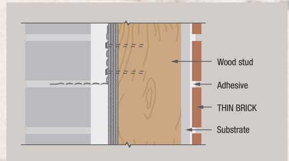
ADHESIVE INTERIOR APPLICATION ON WOOD/STEEL STUD BACKING
